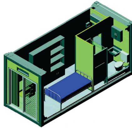
INTERNAL ARRANGEMENT - FRONT ISOMETRIC VIEW
